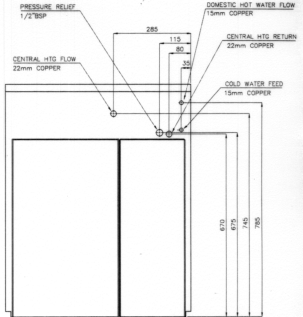
REAR VIEW OF COMBI 65
