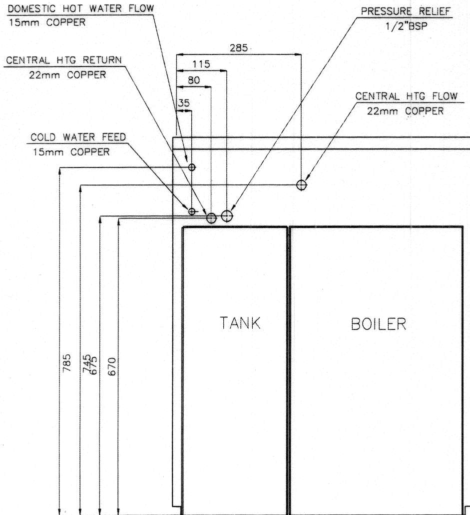
FRONT VIEW OF COMBI 65
